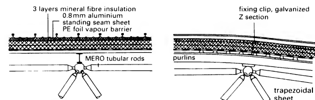
④ Roof skin structure, longitudinal view
